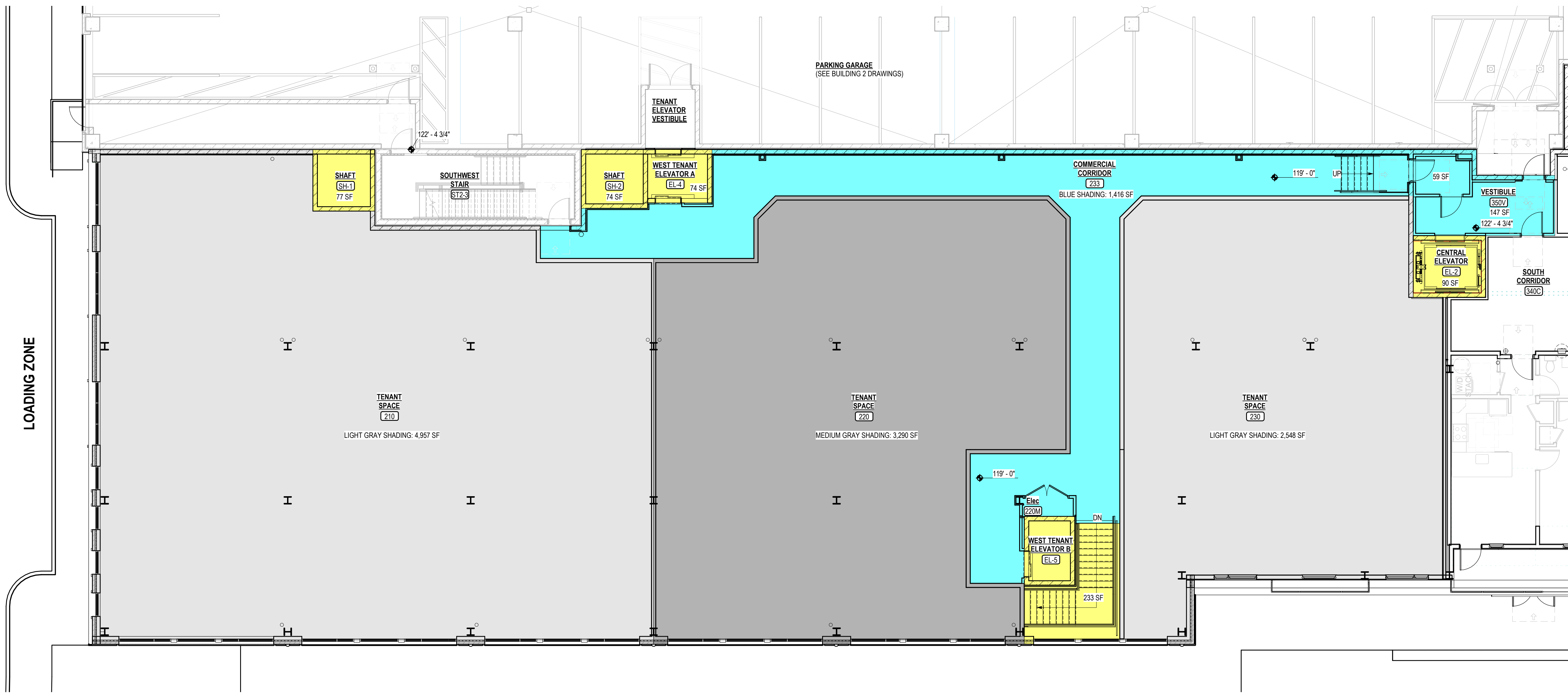
2 west tenant 2nd floor plan L2.13 1/8" = 1'-0"
